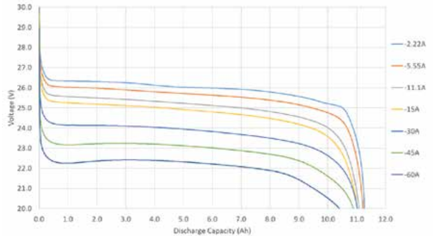
K2B24V11EB Discharge Rates at 23°C
