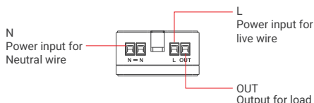
Wire Connection port
