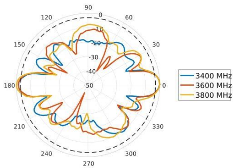
Elevation: 3400 – 3800 MHz
