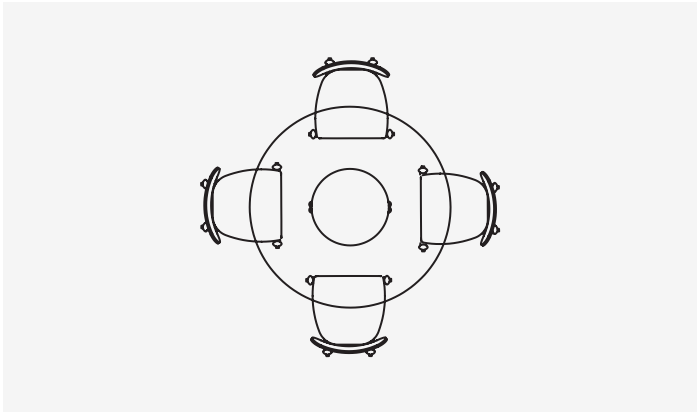
IE120 | Seating for 4 chairs Chair Shown RY49 | Rye — 490L x 470D x 798H x 450SH(mm) 19L x 18L x 30D x 18SH (inches)
