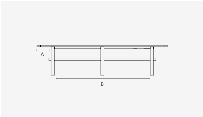
Angle 1 | A Leg Inset Short Edge | B Space Between Legs
