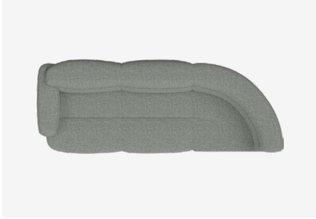
VA299CL — 2990L x 1100D x 680H x 380SH (mm) 118L x 43D x 30H x 15SH (inches)
