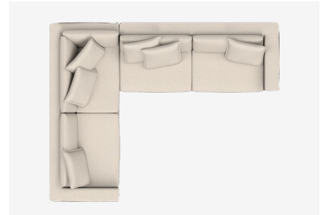
Modular C | SU290CL + SU257R 3680L x 2900D x 750H x 410SH (mm) 145L x 114D x 30H x 16SH (inches)
