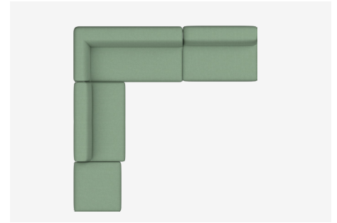
Modular F | MO95P + MO130A + MO192L + MO130LBA 3220L x 3150D x 730H x 3600SH (mm) 127L x 124D x 28H x 14SH (inches)
