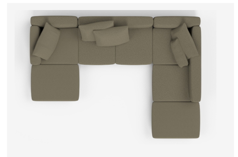
Modular C | ML185R-2 + ML160A + ML265L-2 3680L x 2650D x 680H x 400SH (mm) 145L x 114D x 27H x 16SH (inches)
